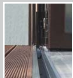
System SF65 bottom running with flush track
